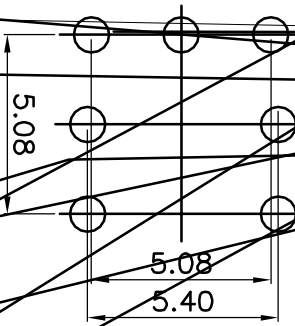
PCB layout (Pattern Side)
